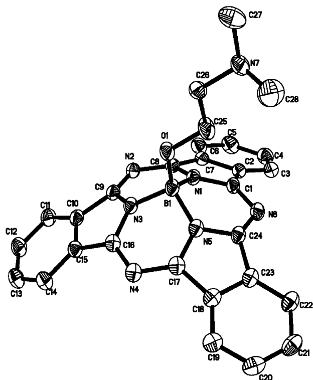
Figure 1. Molecular structure of SPc(OCH 2 CH 2 NMe 2 ) ( 6 ) showing the 30% probability thermal ellipsoids for all non-hydrogen atoms.
