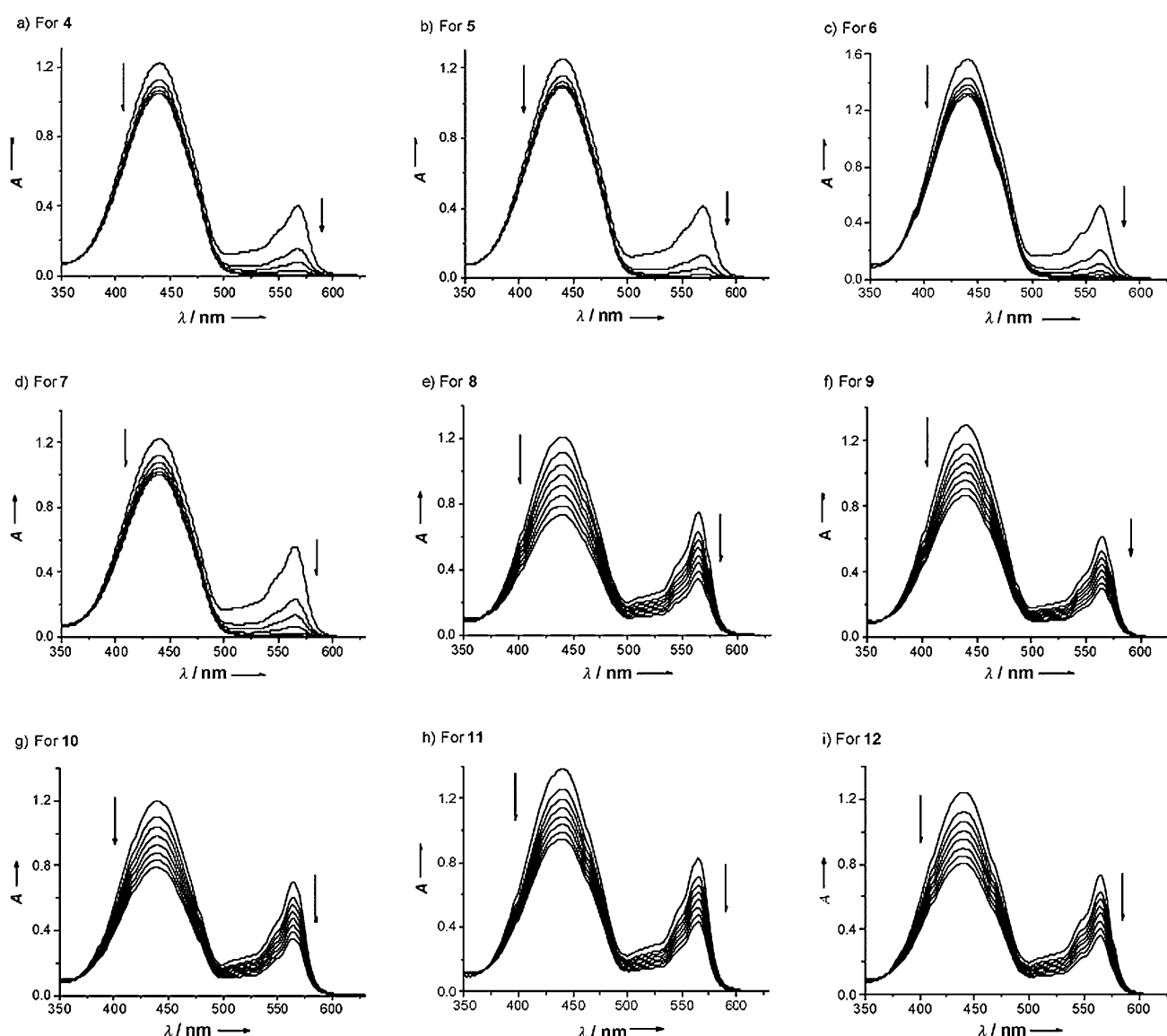
Figure 6. Changes in absorption spectra of mixtures containing 4–12 (8.0 \mu\text{M} ), 0.05% (w/v) Cremophor EL, RNO (25.0 \mu\text{M} ), and imidazole (6.3 mM) in water upon irradiation ( \lambda > 515 nm) with time. The spectra were taken at 3 min intervals. The relative rates of decay of RNO and the photosensitizer can be compared by monitoring the decrease in absorbance at 440 and 564–568 nm, respectively.
