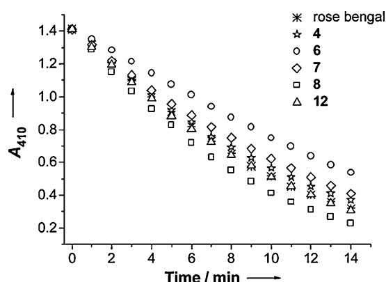
Figure 4. Comparison of the rates of decay of DPBF in EtOH as monitored spectroscopically at 410 nm, using subphthalocyanines 4 , 6–8 , and 12 as the photosensitizers and rose bengal as the reference.
