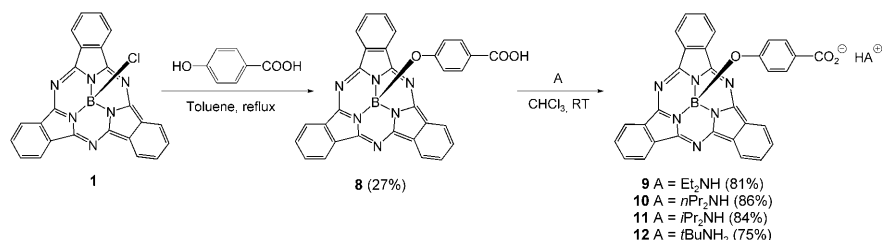
Scheme 3. Synthesis of subphthalocyanines 8–12 .
