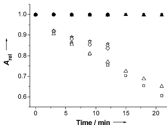
Figure 7. Changes in absorbance of RNO at 440 nm with time [initial [RNO] = 25.0 \mu\text{M} ] using subphthalocyanines 4 (stars), 6 (circles), 7 (diamond), 8 (squares), and 12 (triangles) as the photosensitizers (all at 8 \mu\text{M} ) in water with 0.05 % (w/v) Cremophor EL, both in the absence (closed symbols) and presence (open symbols) of light ( \lambda > 515 nm, 118 mW cm ^{-2} ). The data were taken at 3 min intervals ([imidazole] = 6.3 mM).
