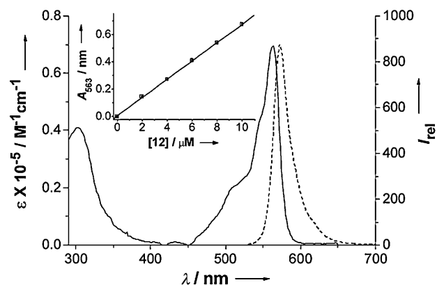
Figure 2. Electronic absorption (—) and fluorescence emission (---) spectra of 12 in DMF (2.0 \mu\text{M} ). The inset plots the Q-band absorbance at 563 nm versus the concentration of 12 , showing that the Beer–Lambert Law is followed.
