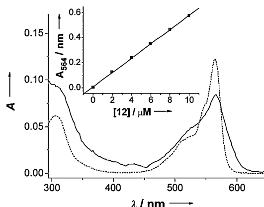
Figure 3. Electronic absorption spectra of 12 in water in the absence (—) and presence of 0.05% (w/v) Cremophor EL (---) (both at 2.0 \mu\text{M} ). The inset plots the Q-band absorbance at 564 nm versus the concentration of 12 .
