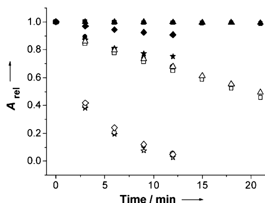
Figure 5. Changes in the Q-band absorbance of 4 (stars), 6 (circles), 7 (diamond), 8 (squares), and 12 (triangles) in water with 0.05% (w/v) Cremophor EL (all at 8.0 \mu\text{M} ) with time, both in the absence (closed symbols) and presence (open symbols) of light ( \lambda > 515 nm, 118 mW cm -2 ). The data were taken at 3 min intervals.
