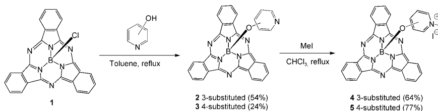
Scheme 1. Synthesis of pyridinium subphthalocyanines 4 and 5 .
