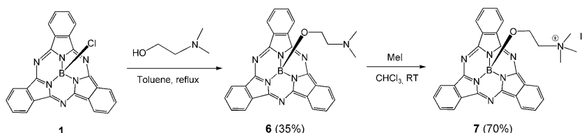
Scheme 2. Synthesis of subphthalocyanines 6 and 7 .
